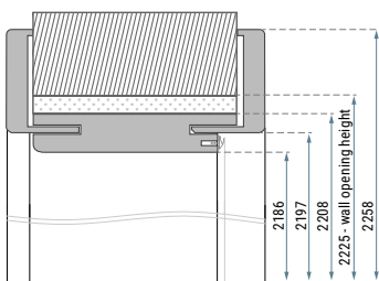
Dimensions of door frame for PN22 door.
