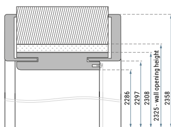
Dimensions of door frame for PN23 door.
